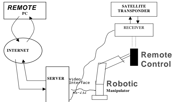
Figure 7: System Schematics
