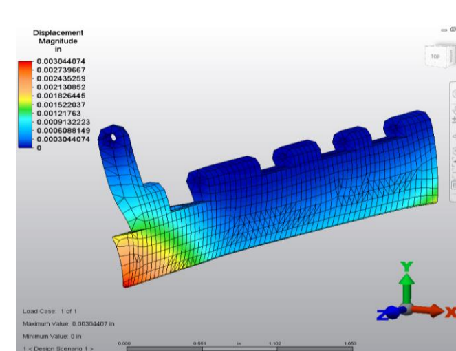
Fig. 5 Deflection profile in nanocoated aircraft inboard flap
