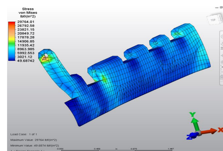
Fig. 4 Stress profile in nanocoated aircraft inboard flap
