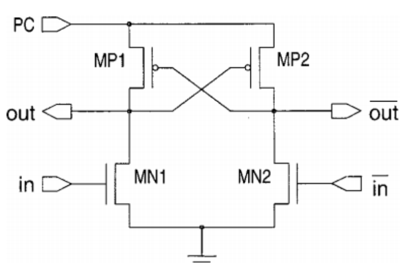
Fig.1. PMOS inverter in TSEL
