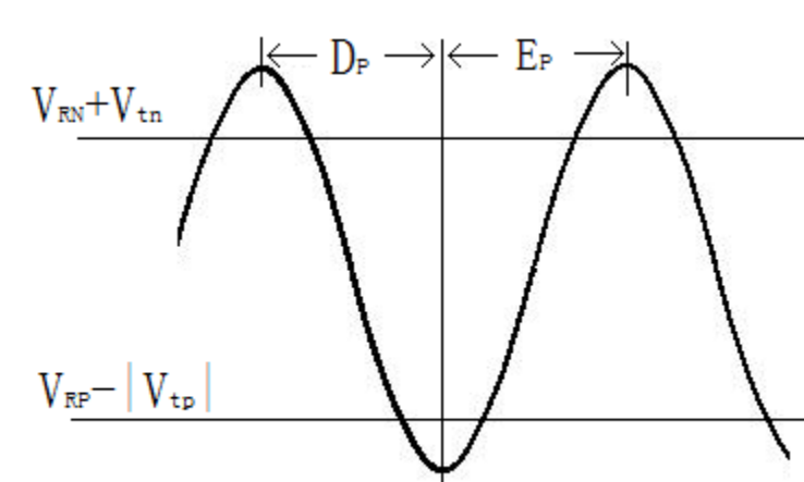
Fig.2. TSEL timing
