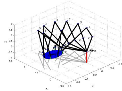
Fig. 6: Manipulator reaching the task points of the Ring Goal
