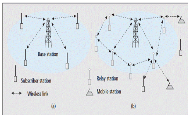
Figure 1. WiMAX network architectures: a) PMP mode; b) mesh mode.
