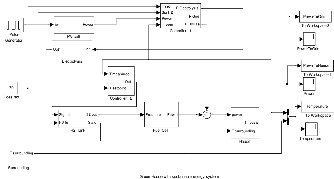
Figure 3 The block diagram of the power system for a green house
