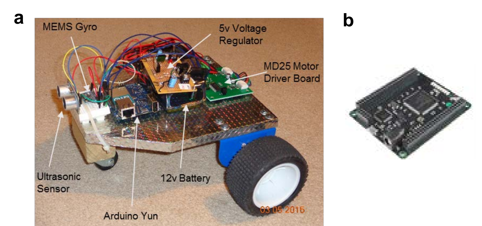
Figure 5: a) The ratbot and b) the Mojo Xilinx FPGA board.
