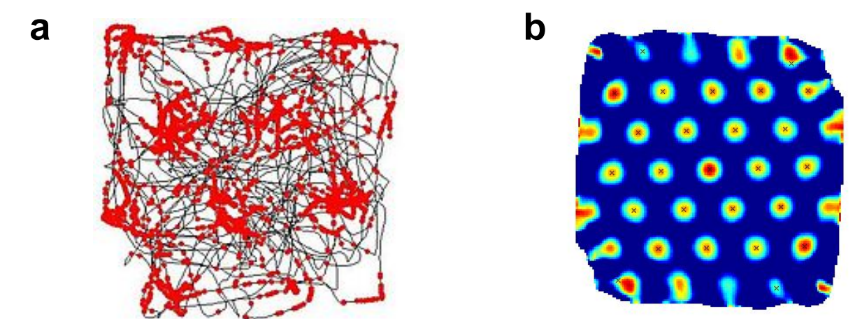
Figure 6: a) Recorded firing locations (red dots) of a single grid cell , as a rat explores (black line) a square, enclosed area. Such recordings are obtained by installing an electrode in a rat's cerebral cortex, where it picks up the firing of a single grid cell as the rat moves around his enclosure. b) The autocorrelogram of the firing data for the grid cell. The hexagonal pattern of the firing locations can be seen in both parts a and b of the figure [3].
