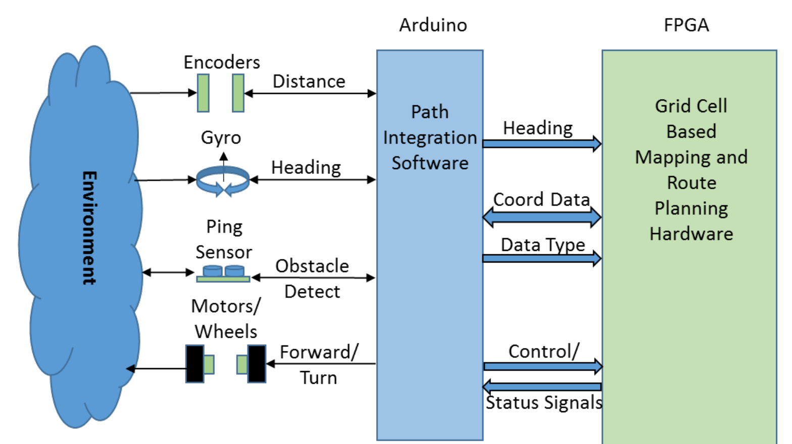
Figure 4: A top level block diagram of the path integration, mapping and route planning circuitry as implemented in the ratbot to simulate the specialized neurobiological navigation cells found in a rat's brain.
