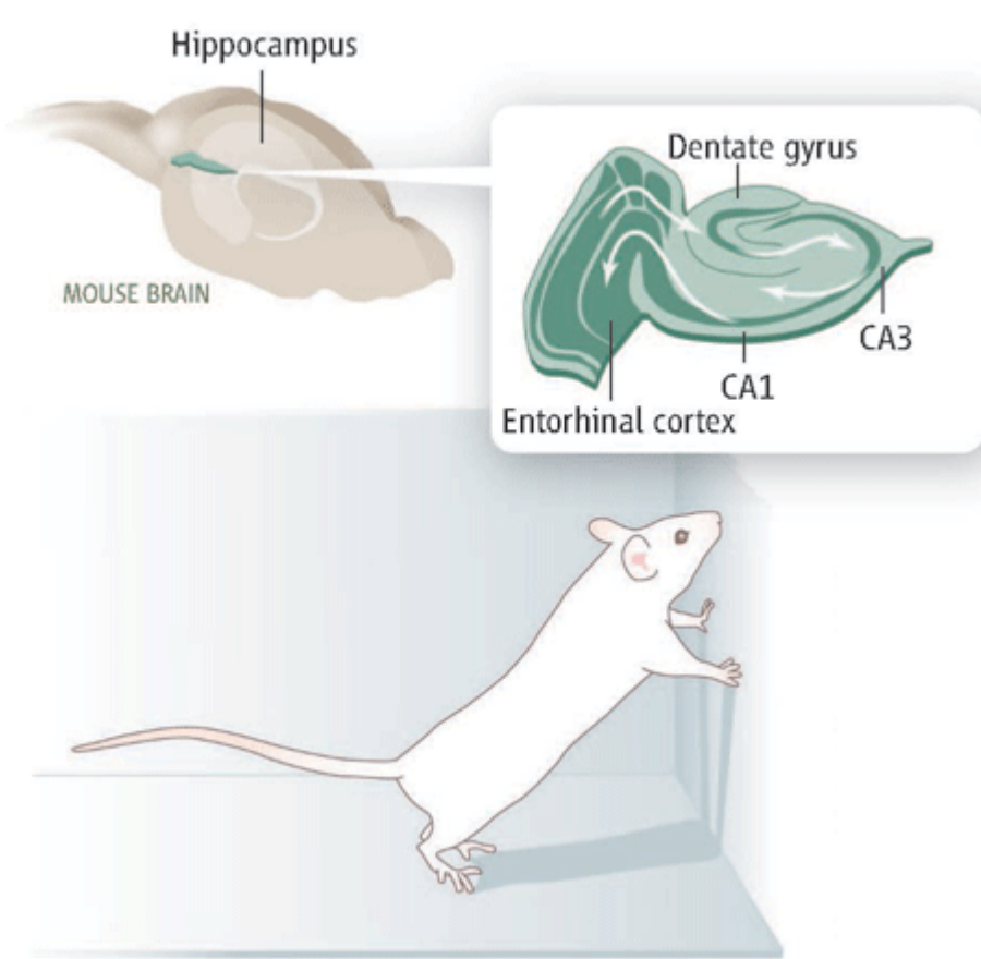
Figure 1: Rodent's hippocampus and entorhinal cortex [4].
